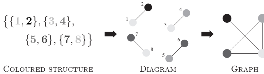
Figure 7.1 A correspondence between a coloured set partition and a graph
